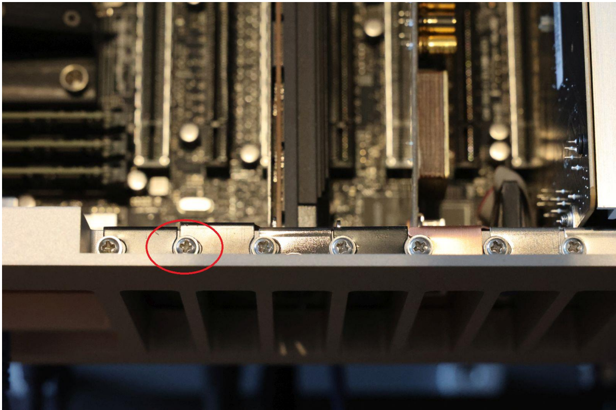
Fig 2a. PCI card fixation screw of an empty slot (Slot 2 is circled in red)
