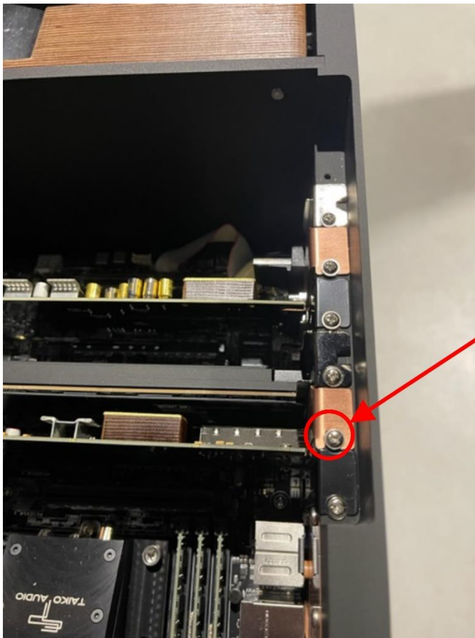
Fig 2b. PCI card fixation screw of an occupied slot (Slot 2 is circled in red)
