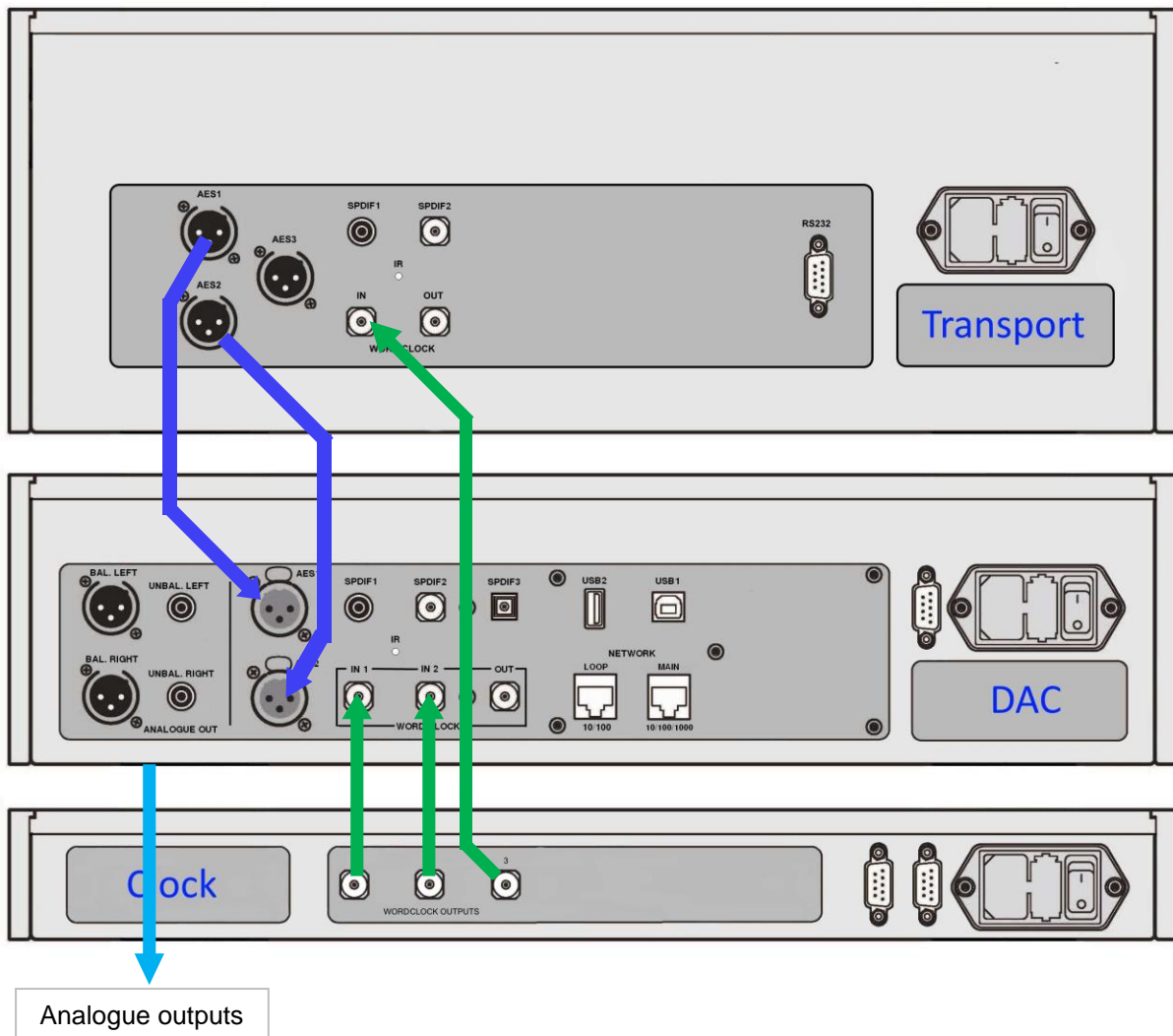
Figure 7 – Using the Rossini DAC, Clock and Transport together
