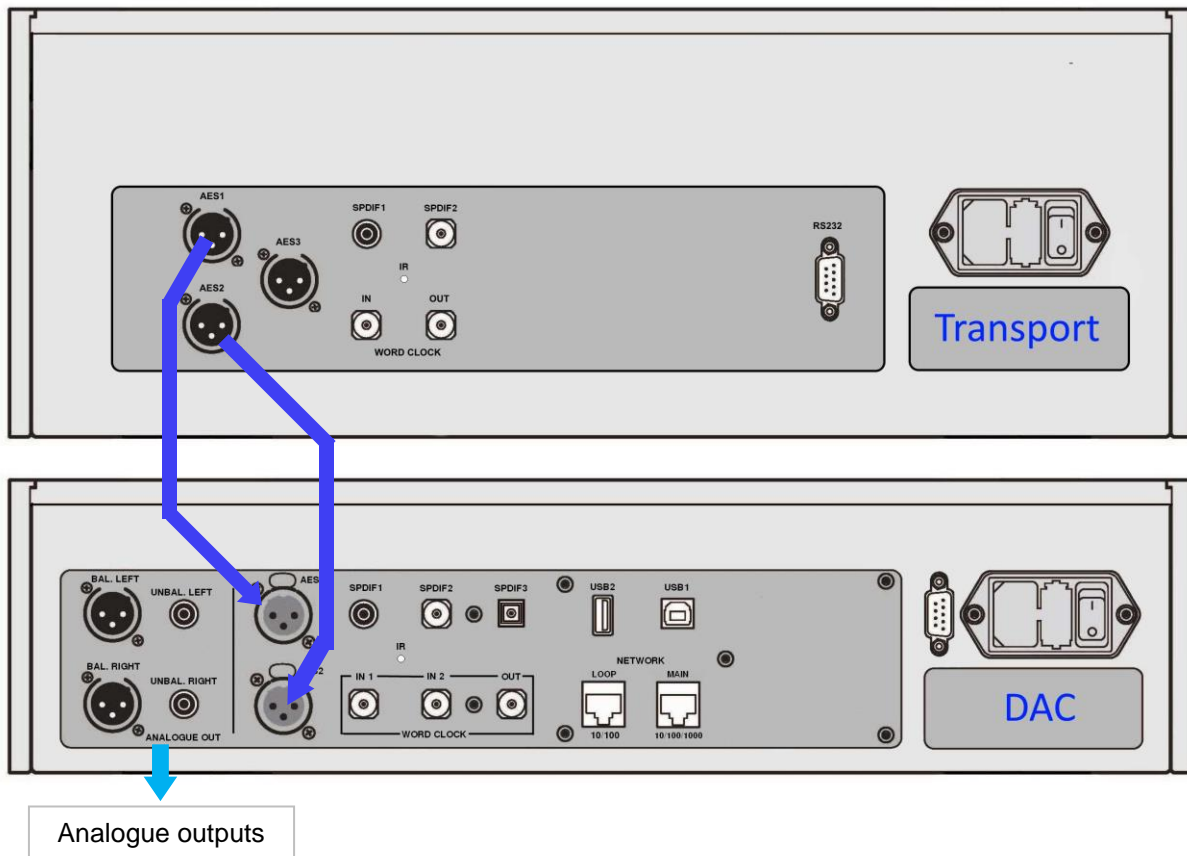
Figure 3 – Using the Rossini DAC with the Rossini CD/SACD Transport
